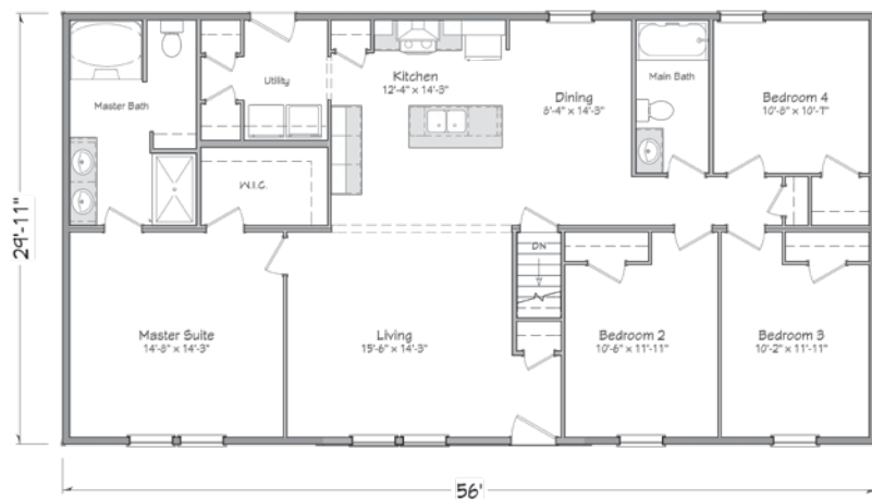
Basement Plan
