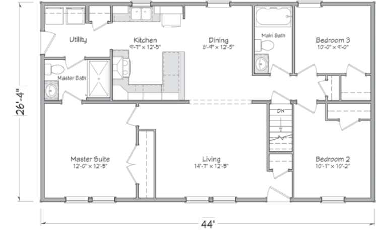
Basement Plan
