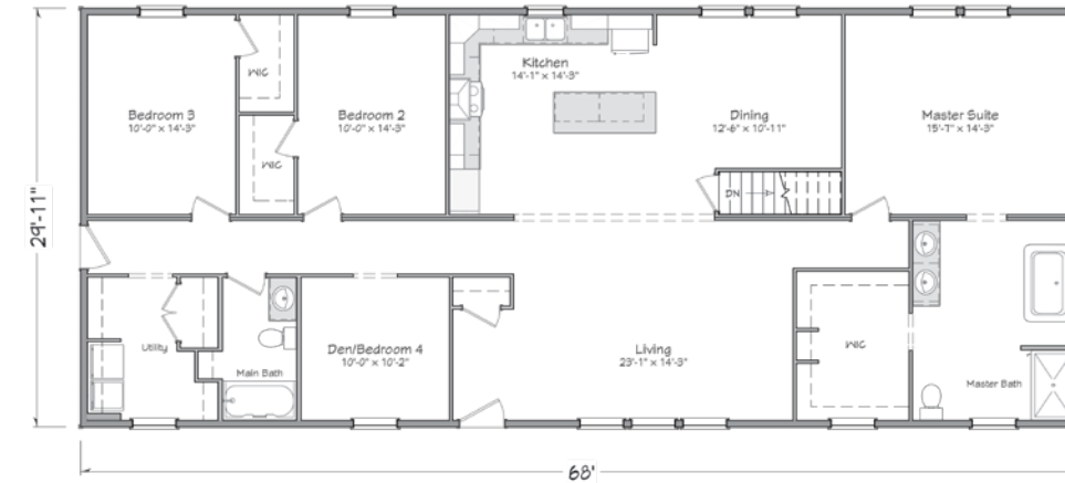
Basement Plan
