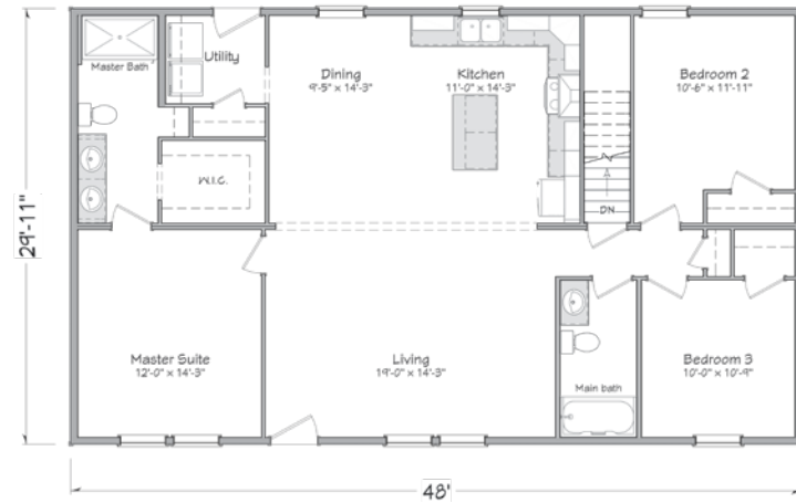
Basement Plan
